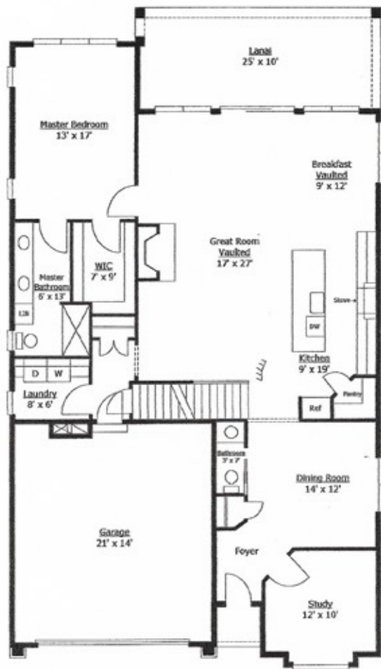
FIRST FLOOR PLAN 1742.33 SQ FT
